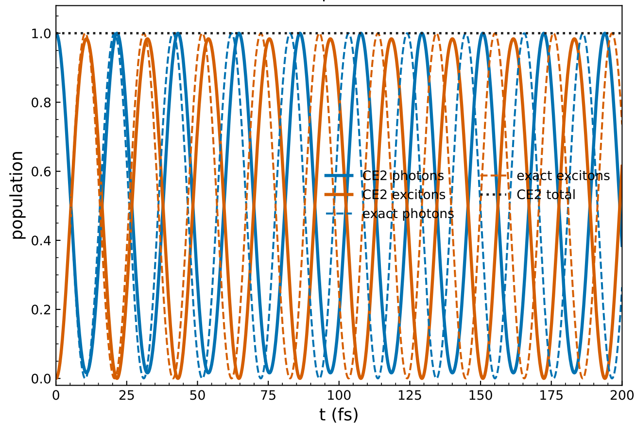
N=5 CE2, one-photon initial state
